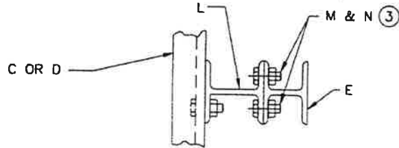
DETAIL-B. PLAN
