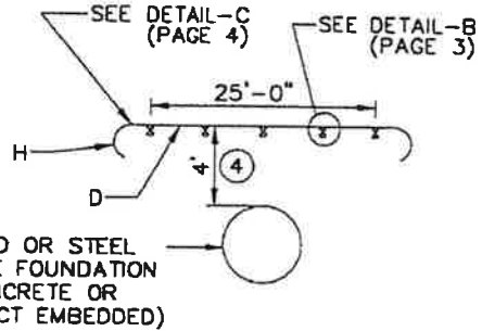
PLAN TYPICAL POLE PROTECTION ON ALL SIDES C9520.22
