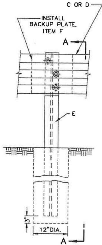
DETAIL-B. ELEVATION
